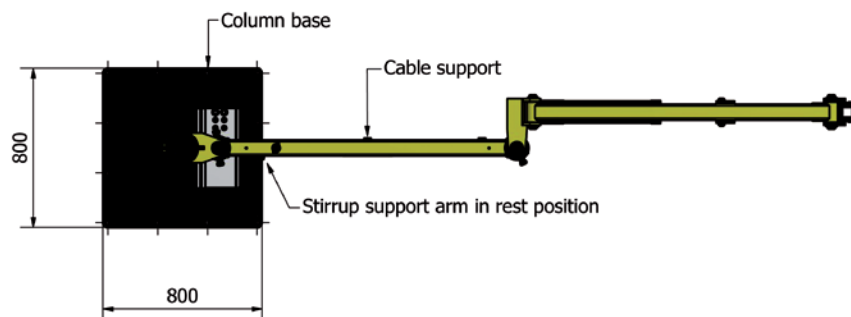
Plan Arm SX
